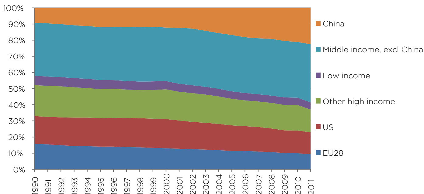
Fig. 1 Historic global GHG emissions 4
